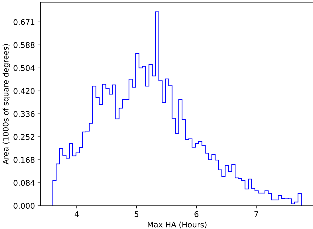
too_elab_heavy_r128_d2_gz_v3.4_10yrs WFD all bands: Max HA
