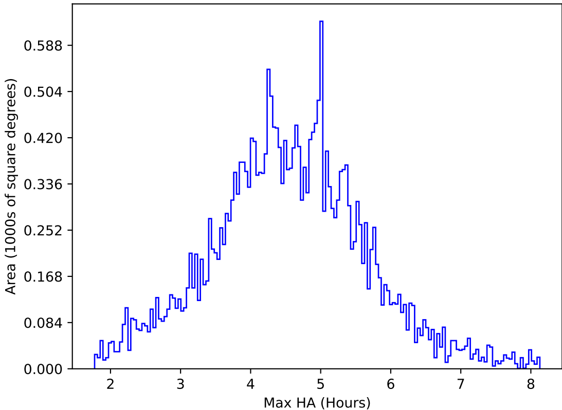
too_elab_heavy_r128_d2_gz_v3.4_10yrs All sky z band: Max HA
