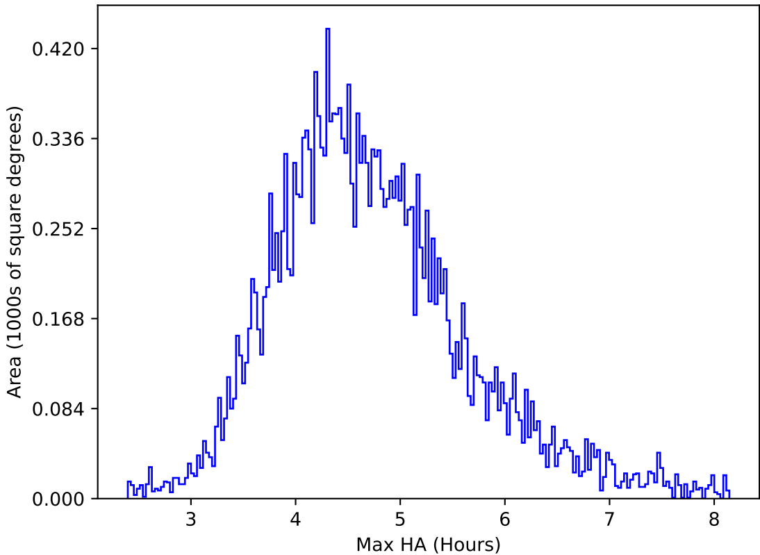
too_elab_heavy_r128_d2_gz_v3.4_10yrs All sky y band: Max HA
