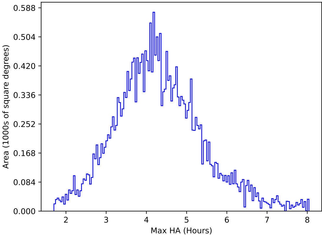
too_elab_heavy_r128_d2_gz_v3.4_10yrs All sky r band: Max HA
