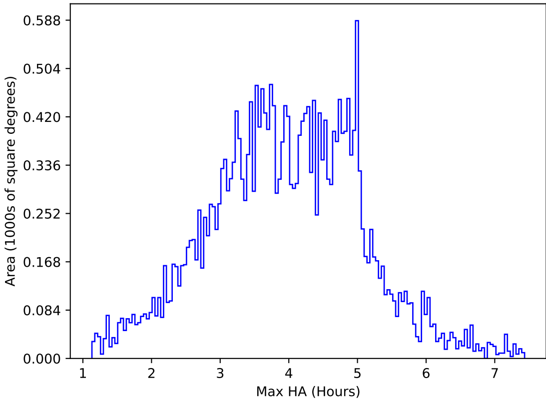
too_elab_heavy_r128_d2_gz_v3.4_10yrs All sky g band: Max HA
