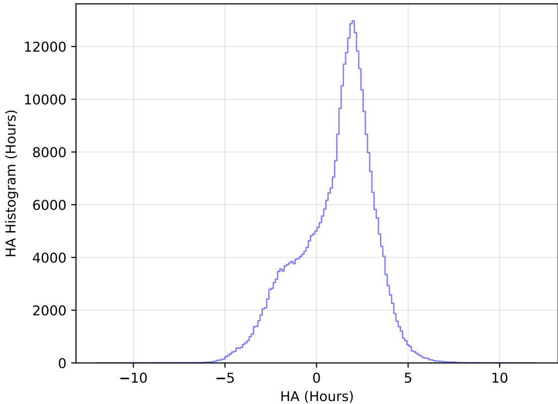
too_elab_heavy_r128_d2_gz_v3.4_10yrs WFD y band: HA Histogram
