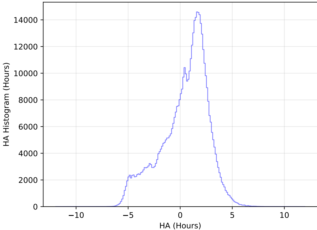
too_elab_heavy_r128_d2_gz_v3.4_10yrs WFD r band: HA Histogram
