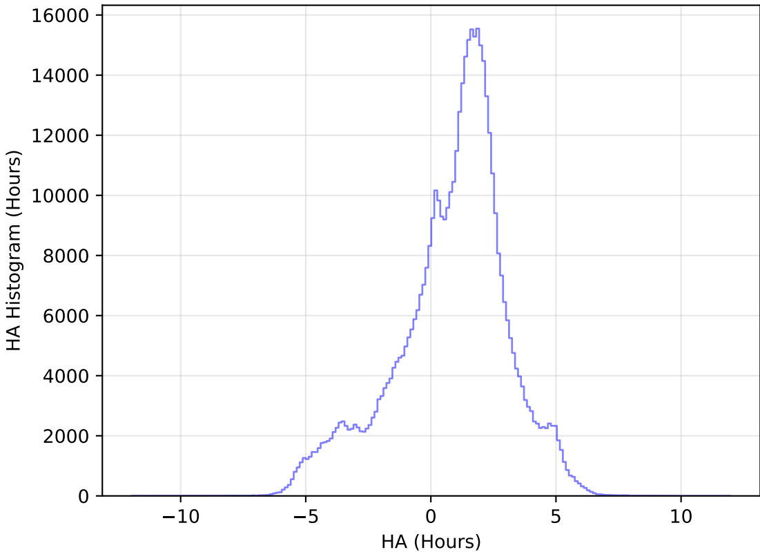
too_elab_heavy_r128_d2_gz_v3.4_10yrs WFD i band: HA Histogram
