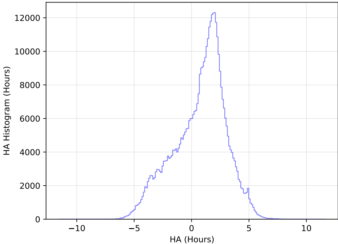
too_elab_heavy_r128_d2_gz_v3.4_10yrs All sky z band: HA Histogram
