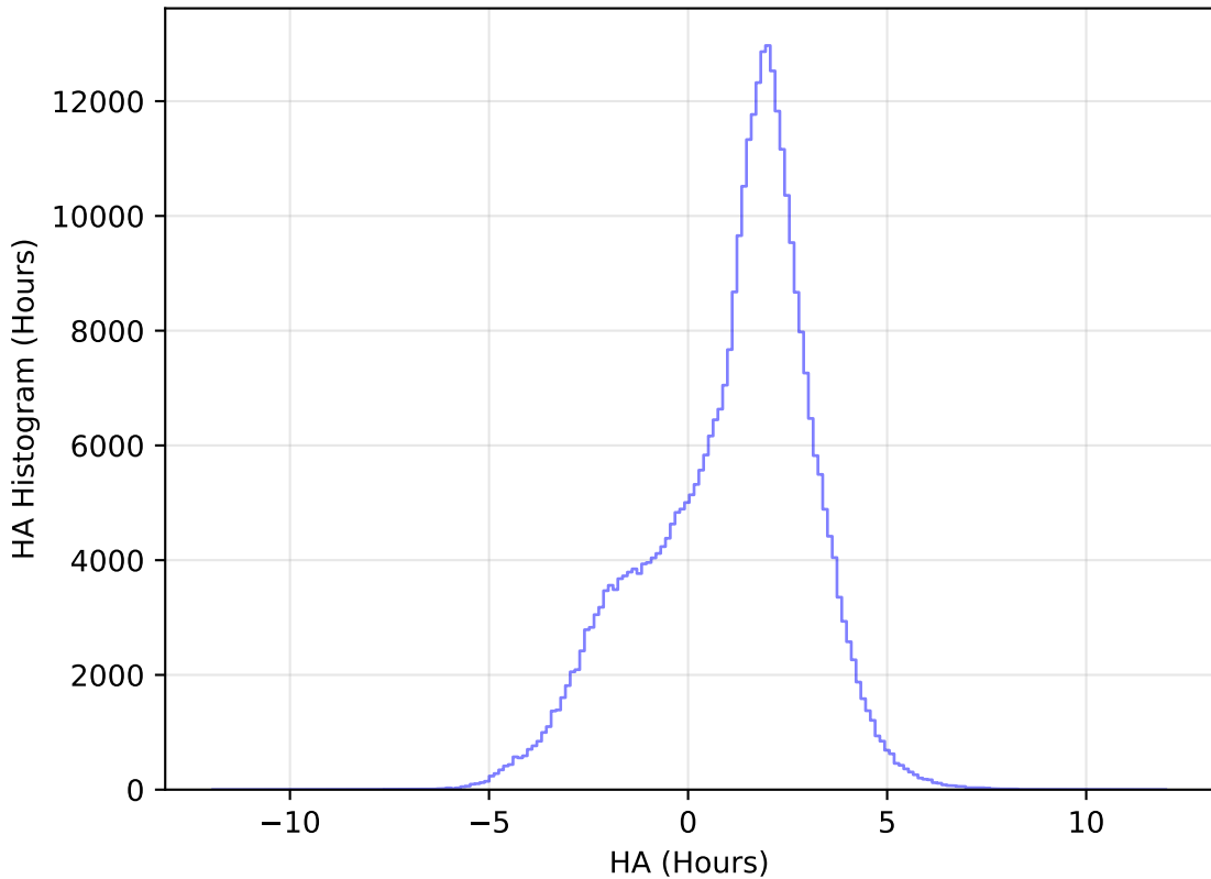
too_elab_heavy_r128_d2_gz_v3.4_10yrs All sky y band: HA Histogram
