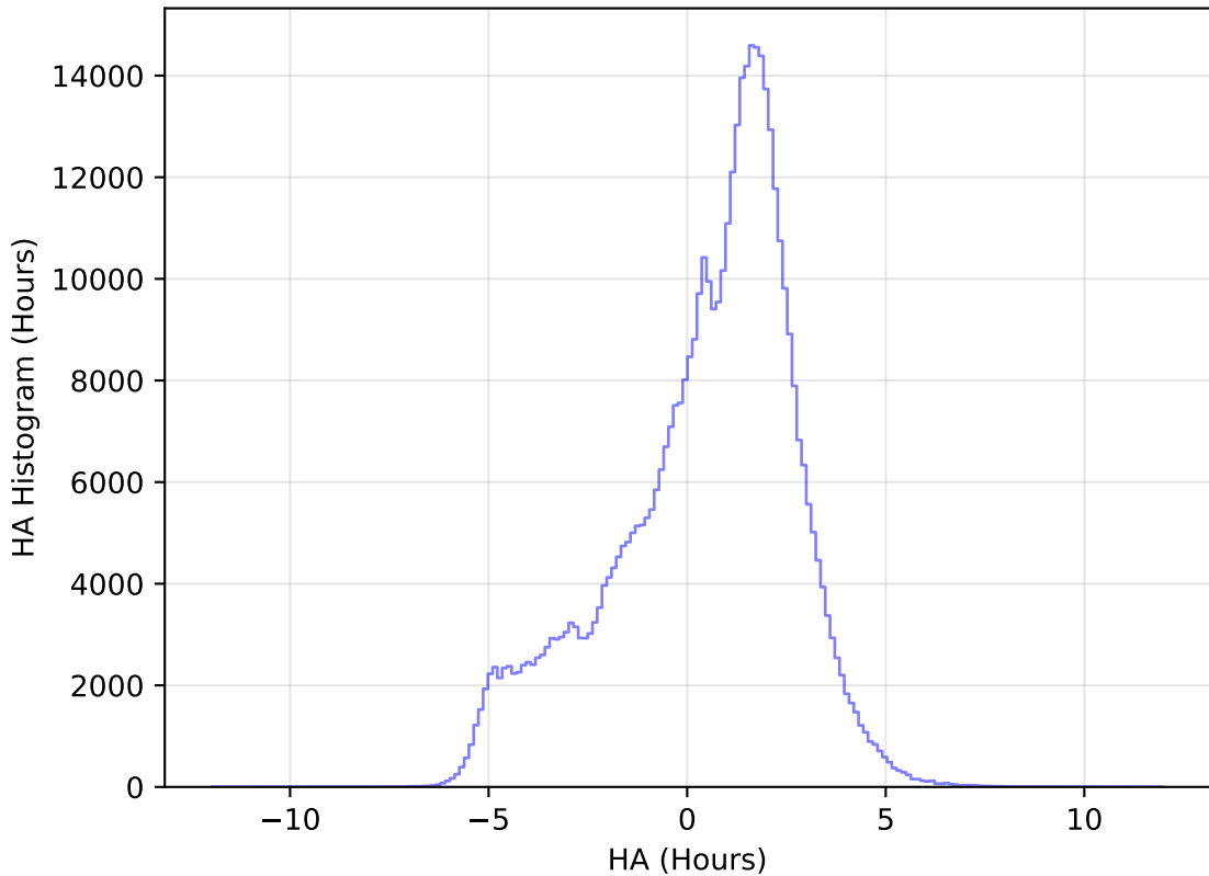
too_elab_heavy_r128_d2_gz_v3.4_10yrs All sky r band: HA Histogram
