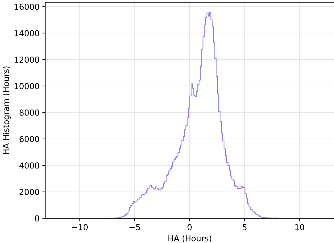
too_elab_heavy_r128_d2_gz_v3.4_10yrs All sky i band: HA Histogram
