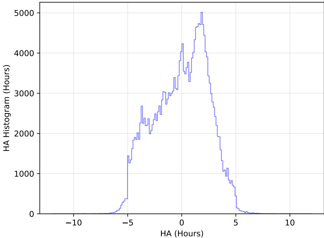
too_elab_heavy_r128_d2_gz_v3.4_10yrs All sky g band: HA Histogram
