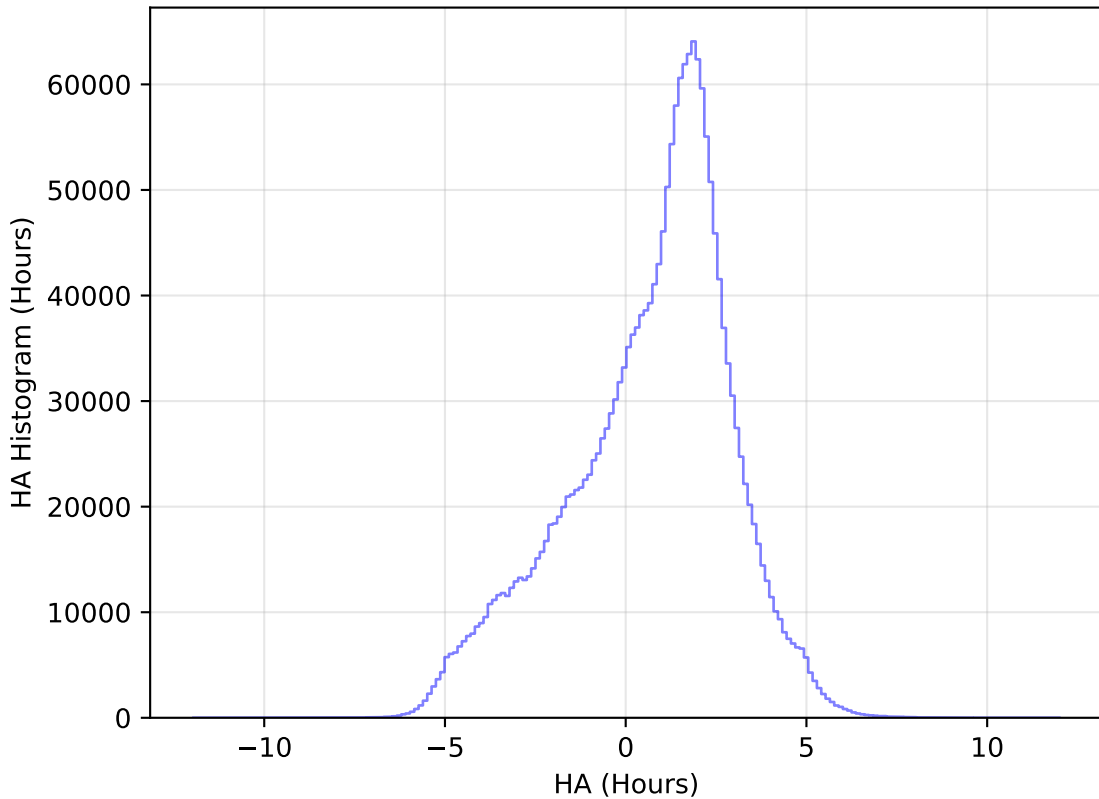
too_elab_heavy_r128_d2_gz_v3.4_10yrs All sky all bands: HA Histogram
