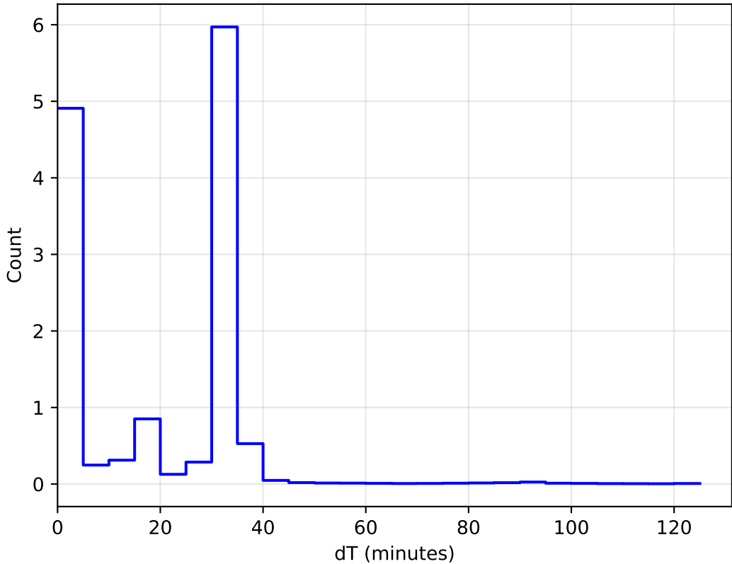
too_elab_heavy_r128_d2_gz_v3.4_10yrs All sky: DeltaT Histogram 1e6
