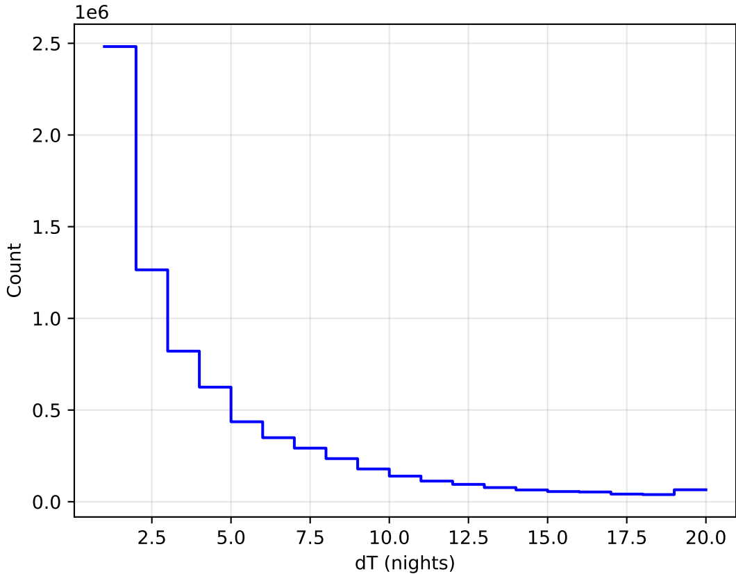
too_elab_heavy_r128_d2_gz_v3.4_10yrs WFD all bands: DeltaNight Histogram
