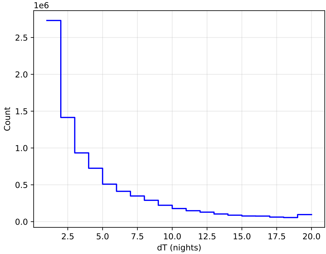
too_elab_heavy_r128_d2_gz_v3.4_10yrs All sky all bands: DeltaNight Histogram
