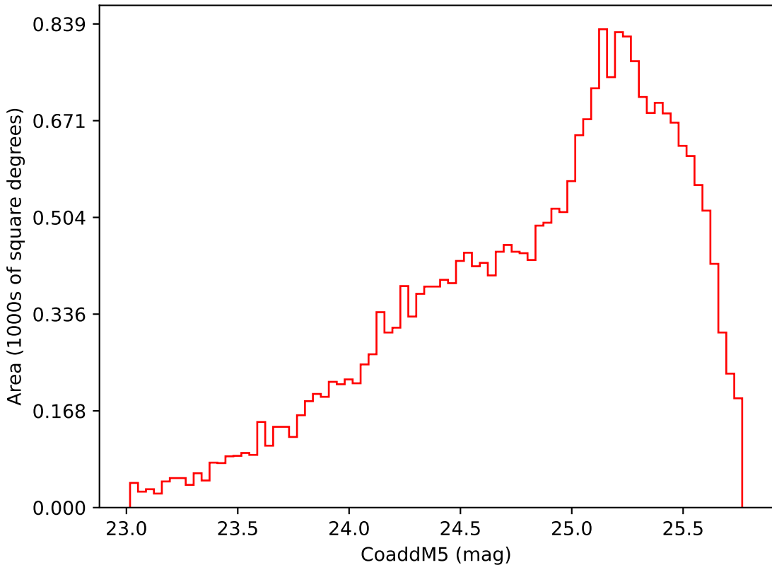
too_elab_heavy_r128_d2_gz_v3.4_10yrs Yr 3-4 i band: CoaddM5
