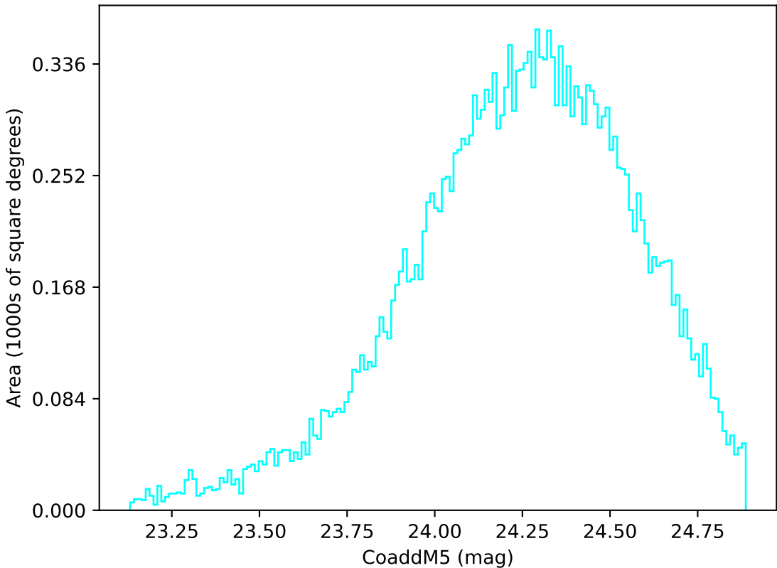
too_elab_heavy_r128_d2_gz_v3.4_10yrs Yr 1 u band: CoaddM5
