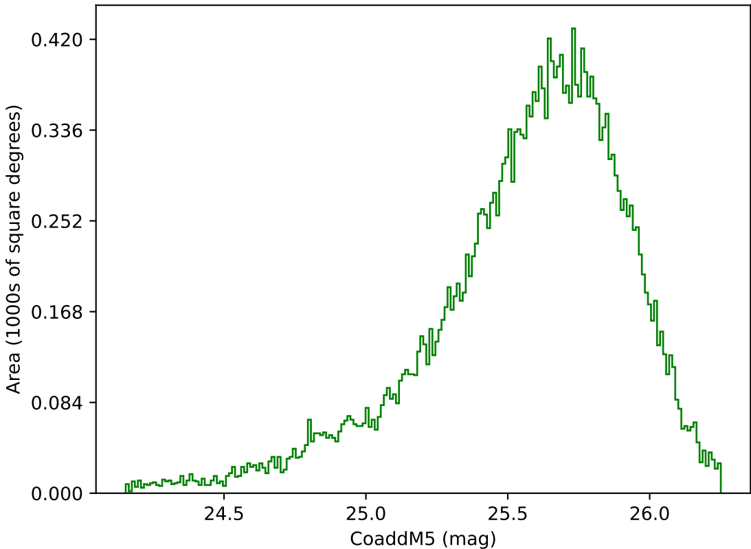
too_elab_heavy_r128_d2_gz_v3.4_10yrs Yr 1 g band: CoaddM5
