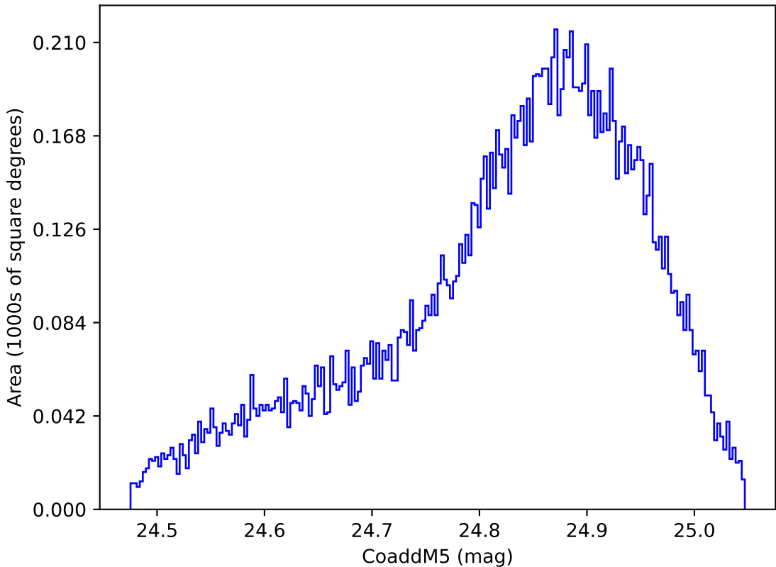
too_elab_heavy_r128_d2_gz_v3.4_10yrs WFD y band: CoaddM5
