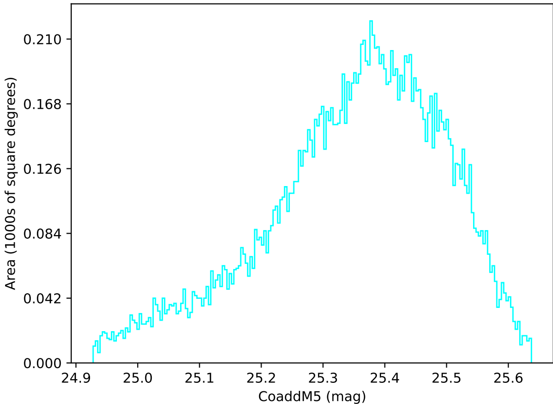
too_elab_heavy_r128_d2_gz_v3.4_10yrs WFD u band: CoaddM5
