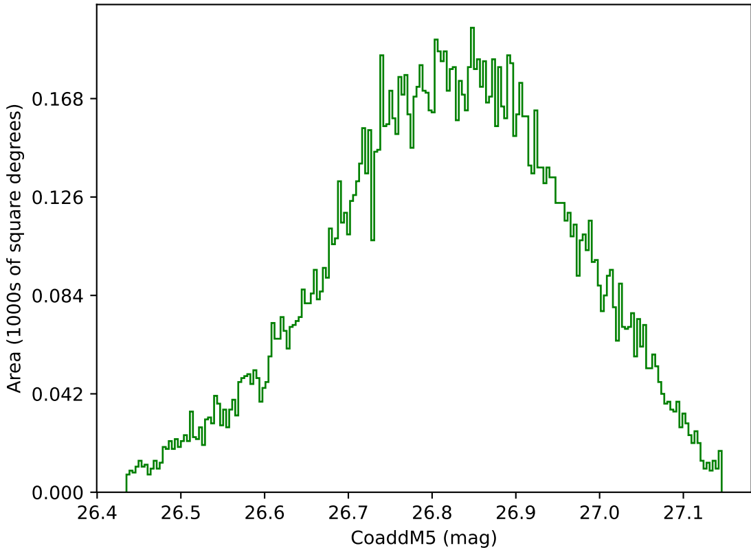
too_elab_heavy_r128_d2_gz_v3.4_10yrs WFD g band: CoaddM5
