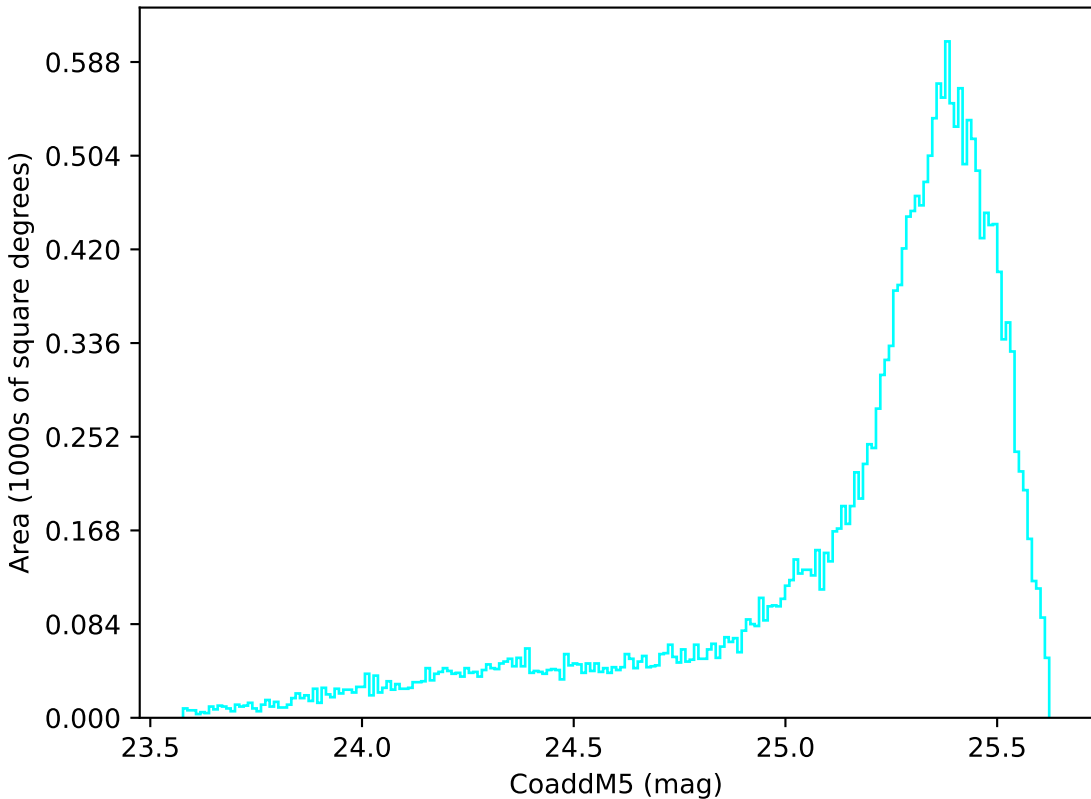
too_elab_heavy_r128_d2_gz_v3.4_10yrs All sky u band: CoaddM5
