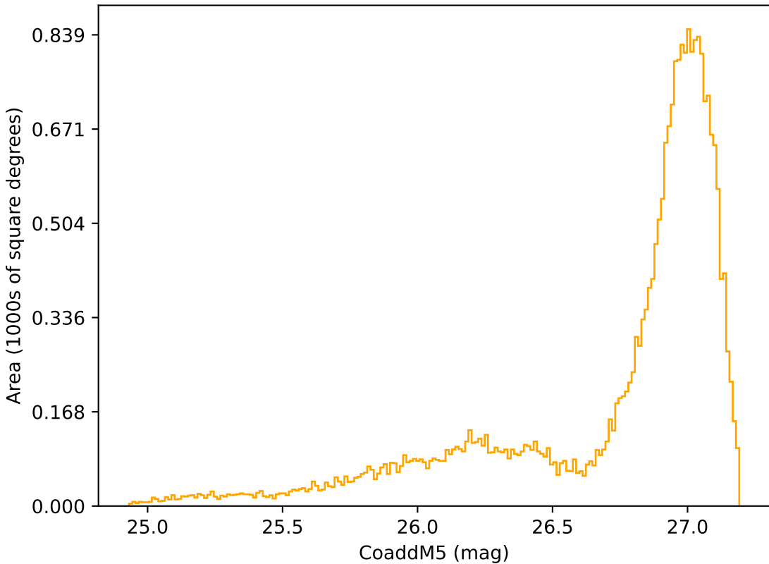
too_elab_heavy_r128_d2_gz_v3.4_10yrs All sky r band: CoaddM5
