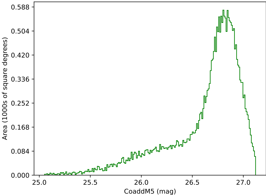
too_elab_heavy_r128_d2_gz_v3.4_10yrs All sky g band: CoaddM5
