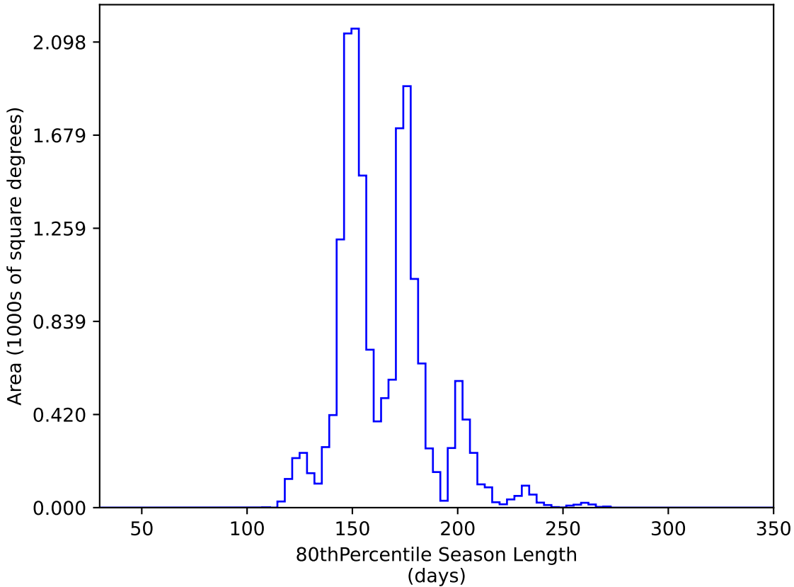
too_elab_heavy_r128_d2_gz_v3.4_10yrs WFD y band: 80thPercentile Season Length
