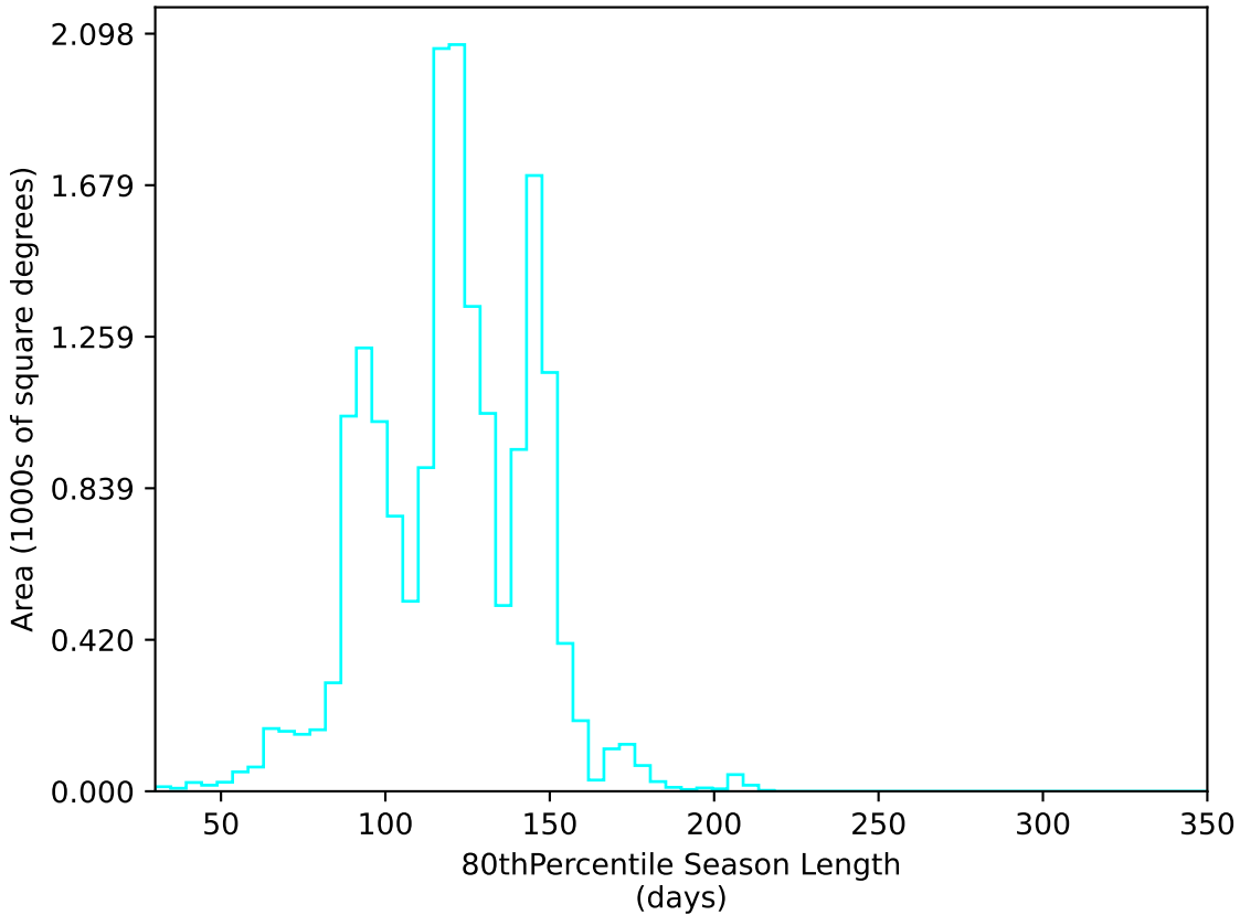
too_elab_heavy_r128_d2_gz_v3.4_10yrs WFD u band: 80thPercentile Season Length
