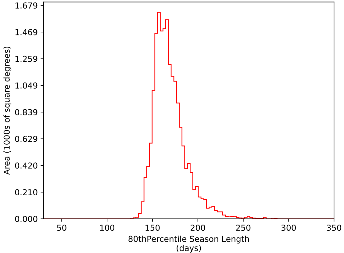
too_elab_heavy_r128_d2_gz_v3.4_10yrs WFD i band: 80thPercentile Season Length
