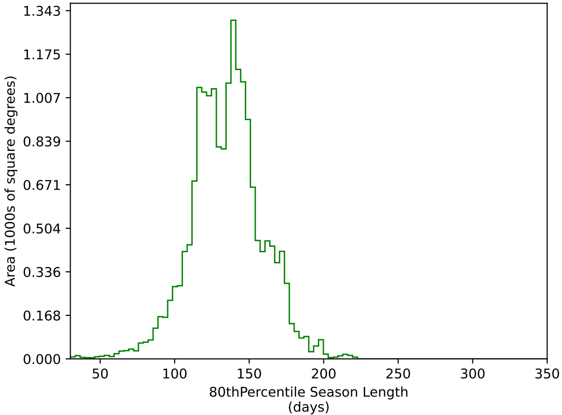
too_elab_heavy_r128_d2_gz_v3.4_10yrs WFD g band: 80thPercentile Season Length
