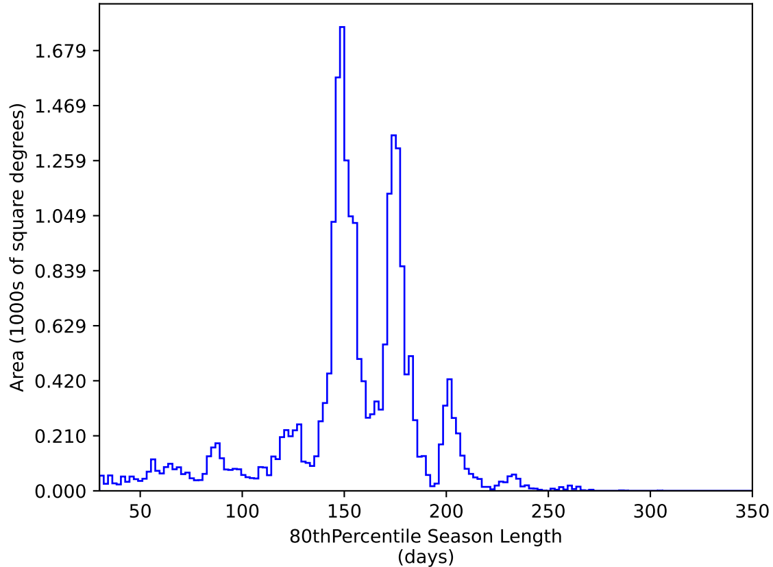
too_elab_heavy_r128_d2_gz_v3.4_10yrs All sky y band: 80thPercentile Season Length
