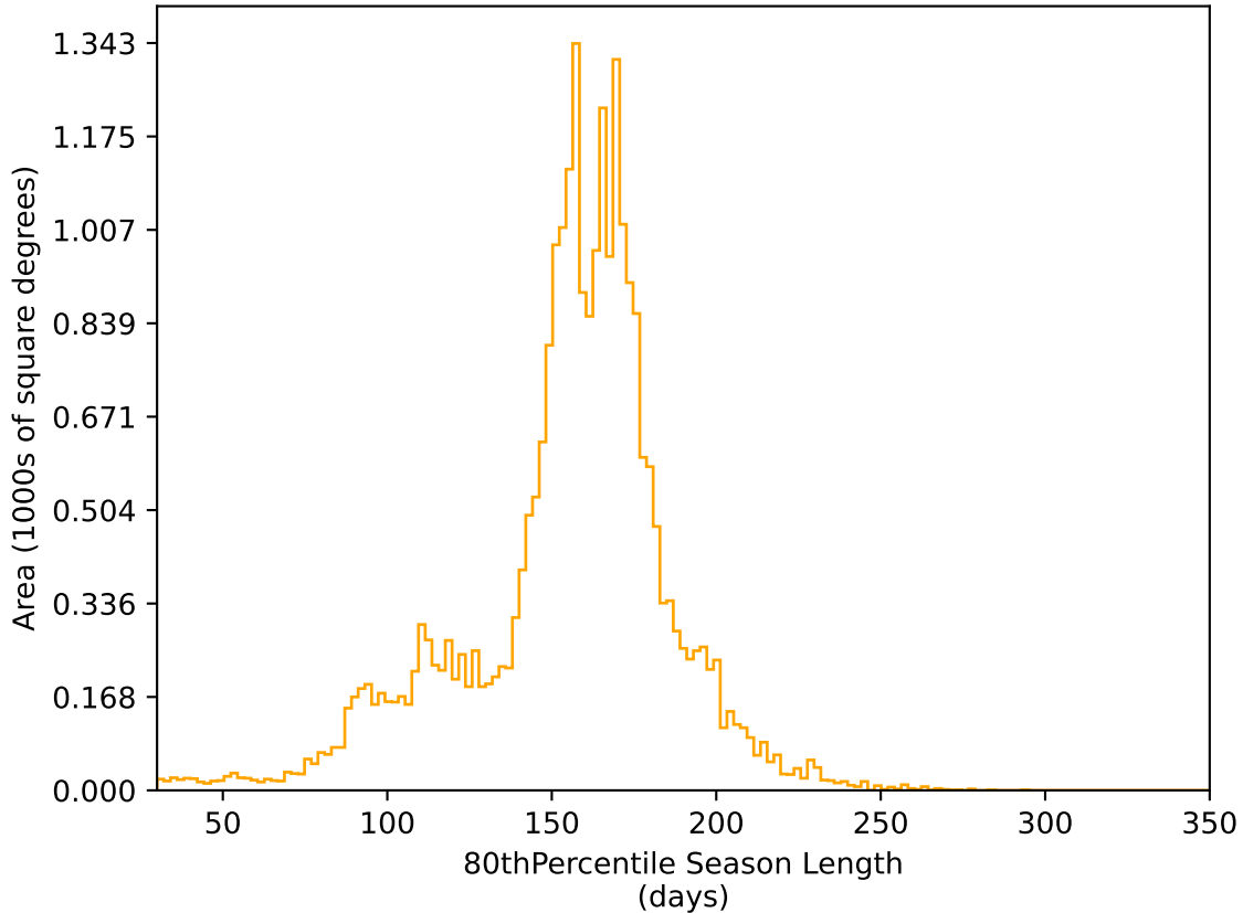
too_elab_heavy_r128_d2_gz_v3.4_10yrs All sky r band: 80thPercentile Season Length
