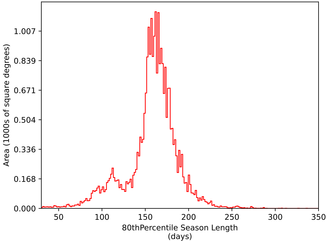
too_elab_heavy_r128_d2_gz_v3.4_10yrs All sky i band: 80thPercentile Season Length
