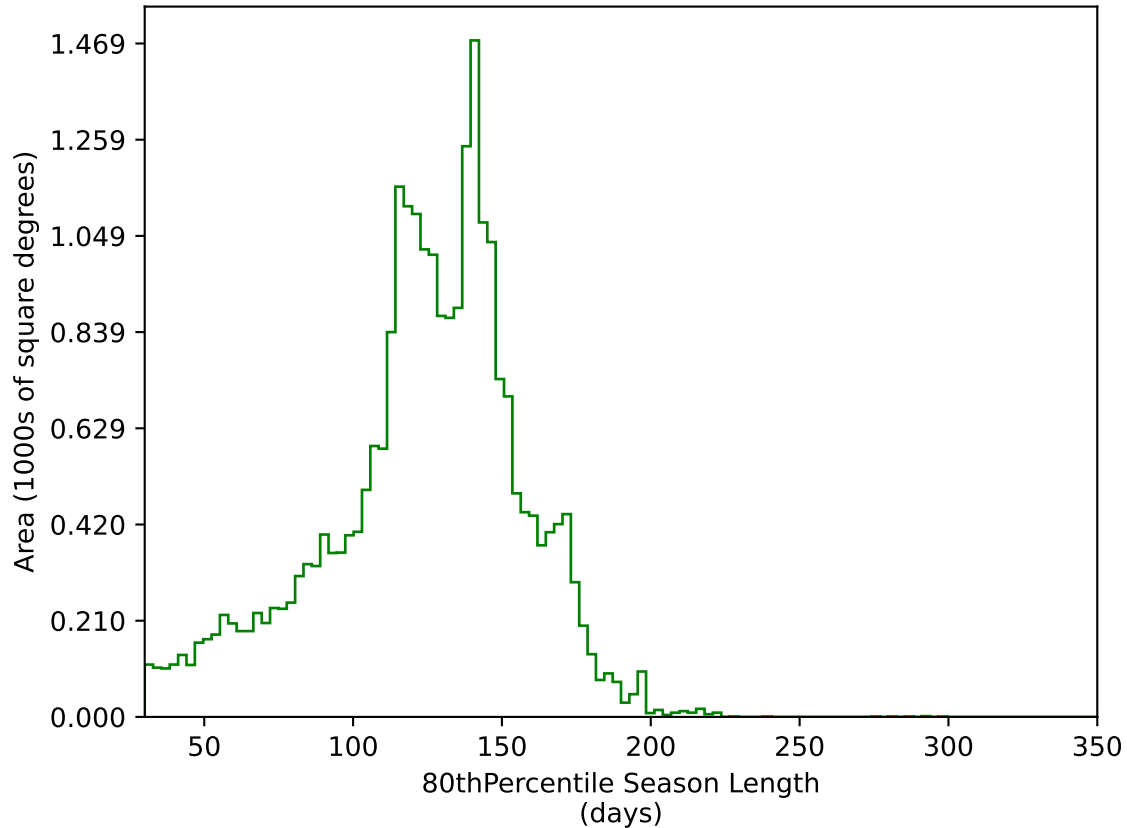
too_elab_heavy_r128_d2_gz_v3.4_10yrs All sky g band: 80thPercentile Season Length
