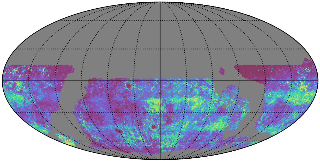
too_elab_heavy_r128_d2_gz_v3.4_10yrs WFD zy bands: 75th Percentile Intranight Timespan
