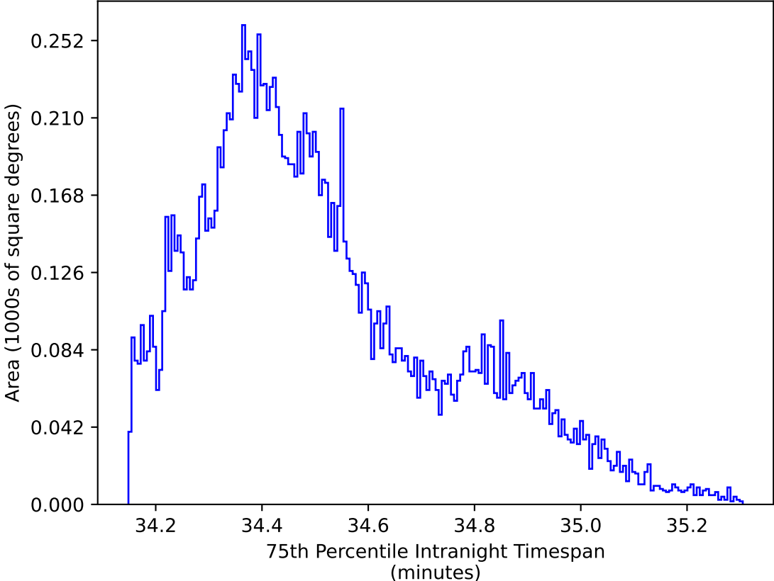
too_elab_heavy_r128_d2_gz_v3.4_10yrs WFD zy bands: 75th Percentile Intranight Timespan
