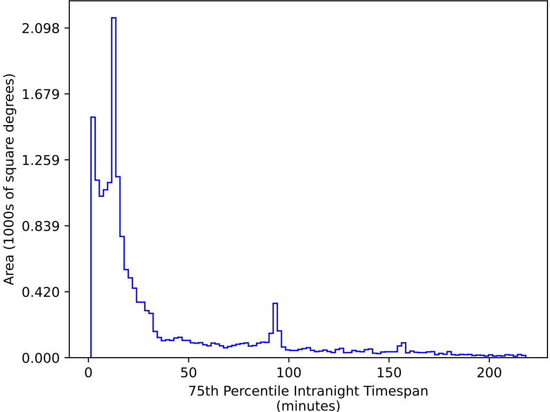
too_elab_heavy_r128_d2_gz_v3.4_10yrs WFD z band: 75th Percentile Intranight Timespan
