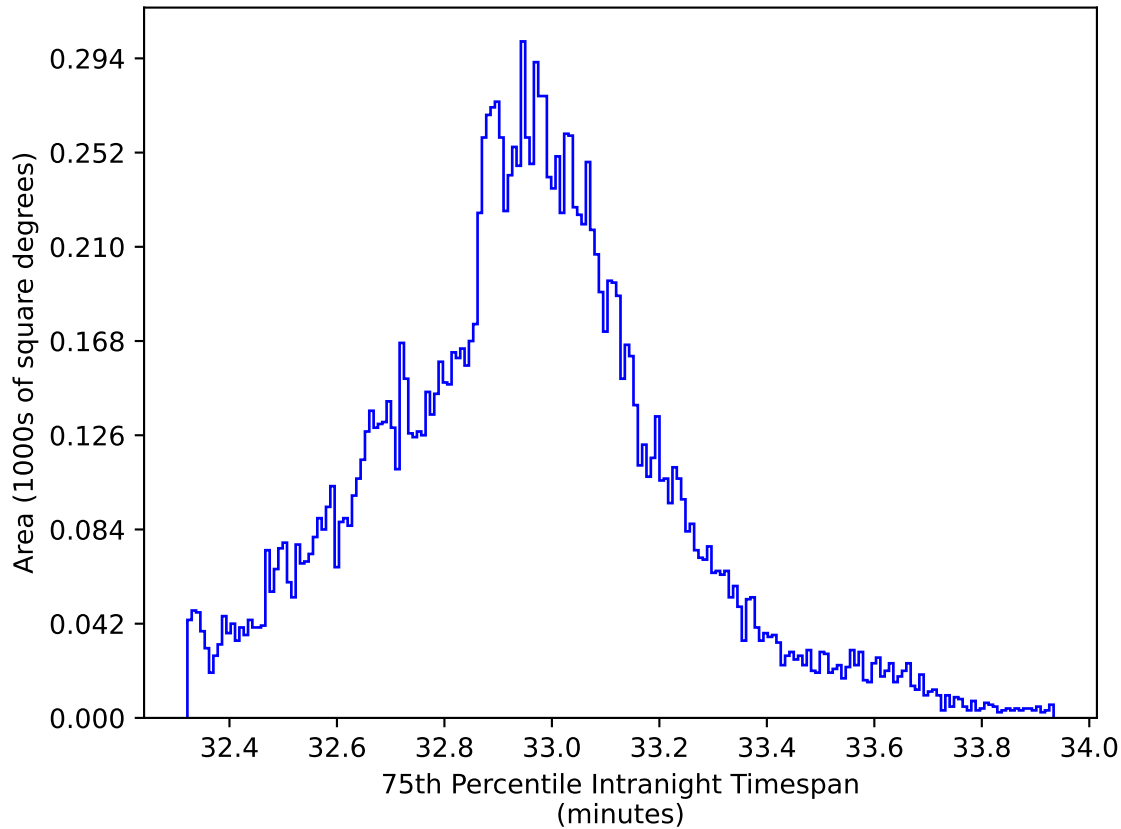
too_elab_heavy_r128_d2_gz_v3.4_10yrs WFD y band: 75th Percentile Intranight Timespan
