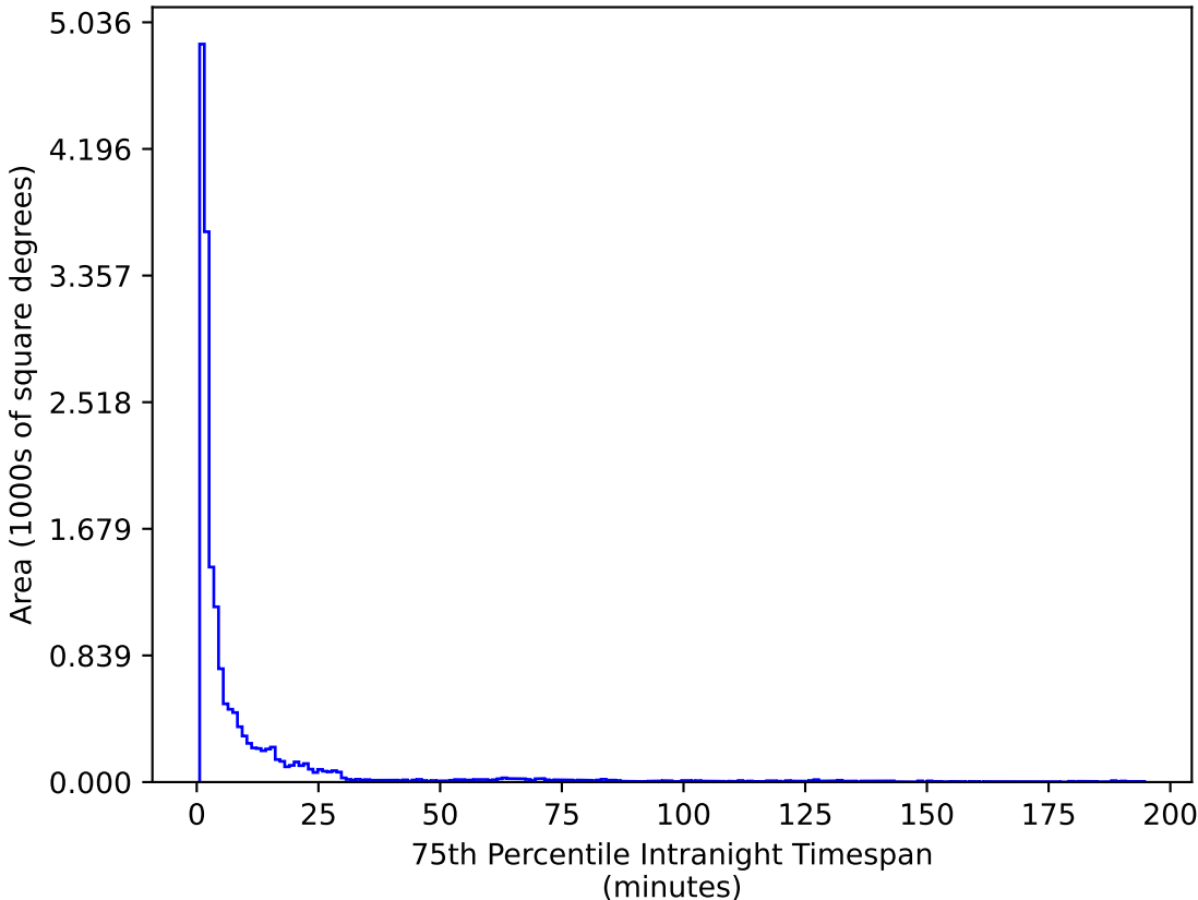
too_elab_heavy_r128_d2_gz_v3.4_10yrs WFD u band: 75th Percentile Intranight Timespan
