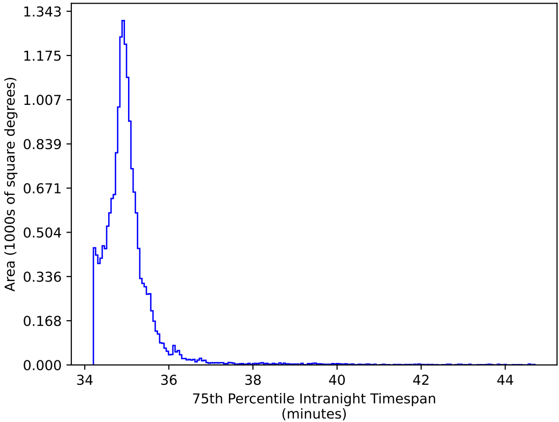
too_elab_heavy_r128_d2_gz_v3.4_10yrs WFD ri bands: 75th Percentile Intranight Timespan
