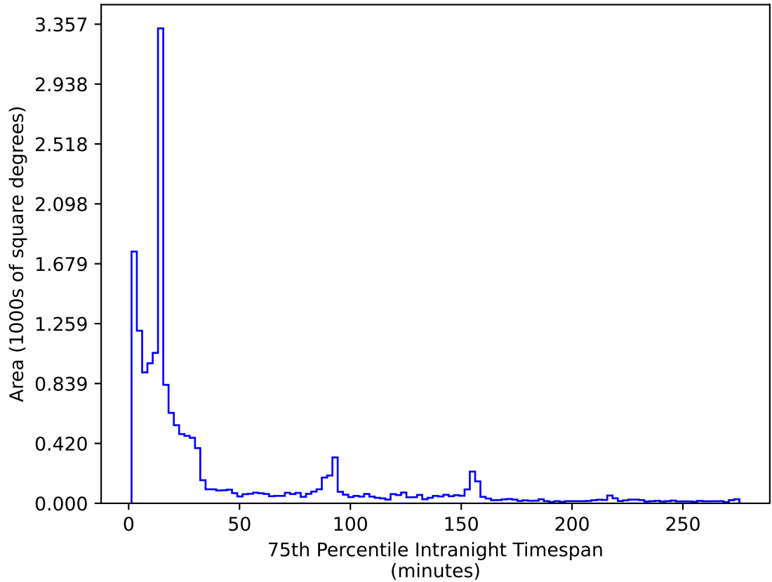
too_elab_heavy_r128_d2_gz_v3.4_10yrs WFD r band: 75th Percentile Intranight Timespan
