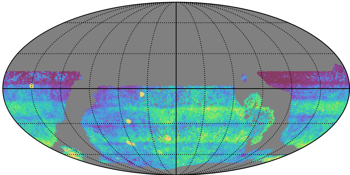
too_elab_heavy_r128_d2_gz_v3.4_10yrs WFD all bands: 75th Percentile Intranight Timespan
