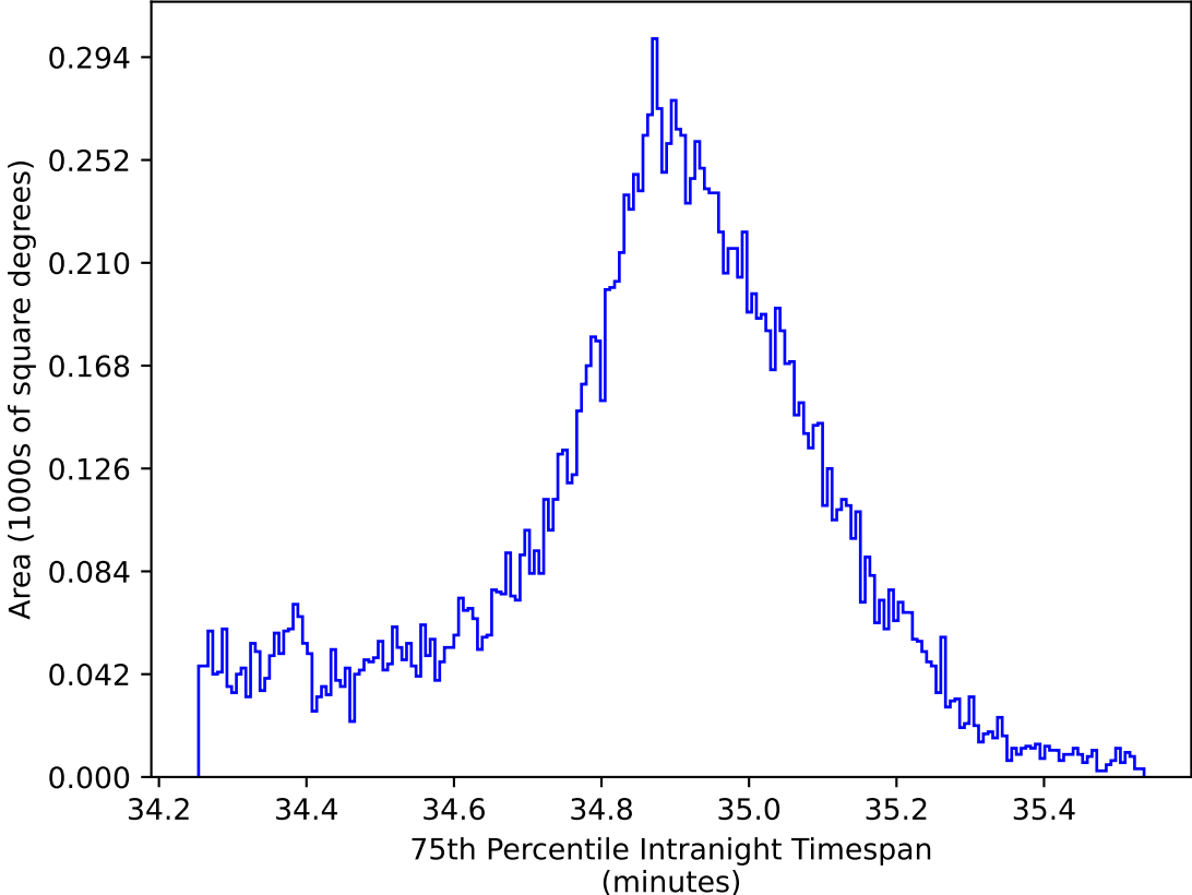
too_elab_heavy_r128_d2_gz_v3.4_10yrs WFD all bands: 75th Percentile Intranight Timespan
