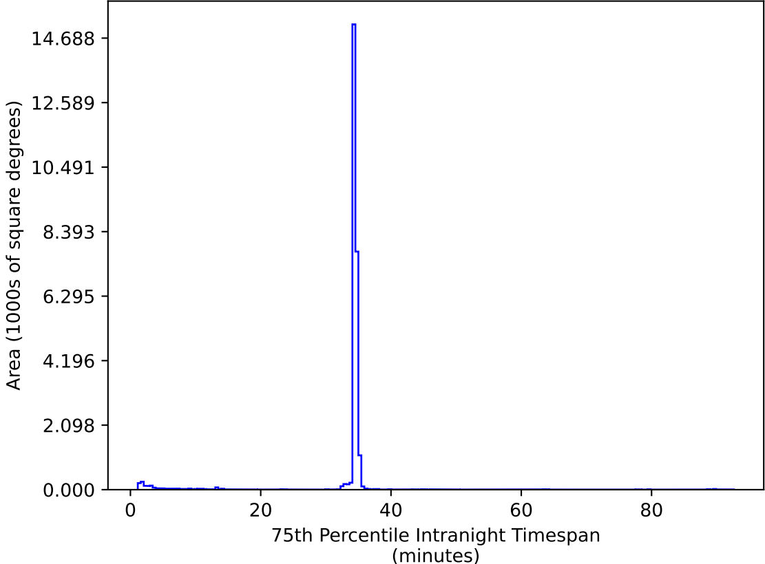
too_elab_heavy_r128_d2_gz_v3.4_10yrs All sky zy bands: 75th Percentile Intranight Timespan
