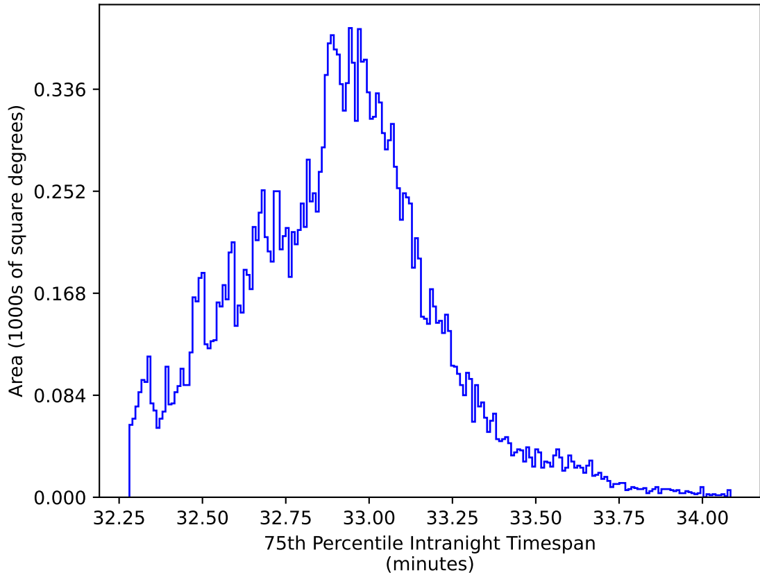
too_elab_heavy_r128_d2_gz_v3.4_10yrs All sky y band: 75th Percentile Intranight Timespan
