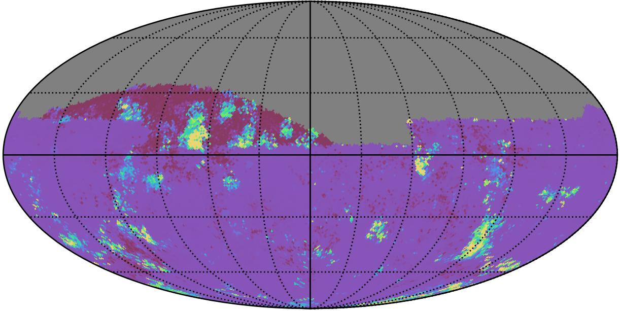
too_elab_heavy_r128_d2_gz_v3.4_10yrs All sky ug bands: 75th Percentile Intranight Timespan
