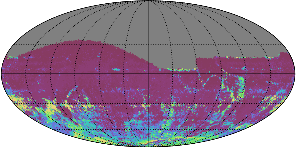
too_elab_heavy_r128_d2_gz_v3.4_10yrs All sky r band: 75th Percentile Intranight Timespan
