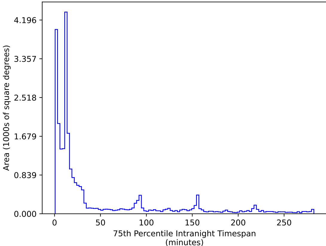
too_elab_heavy_r128_d2_gz_v3.4_10yrs All sky r band: 75th Percentile Intranight Timespan
