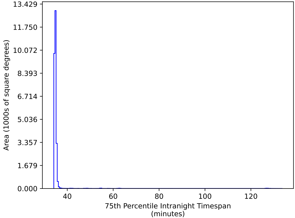
too_elab_heavy_r128_d2_gz_v3.4_10yrs All sky iz bands: 75th Percentile Intranight Timespan
