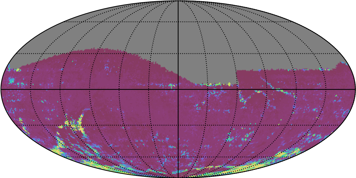
too_elab_heavy_r128_d2_gz_v3.4_10yrs All sky i band: 75th Percentile Intranight Timespan
